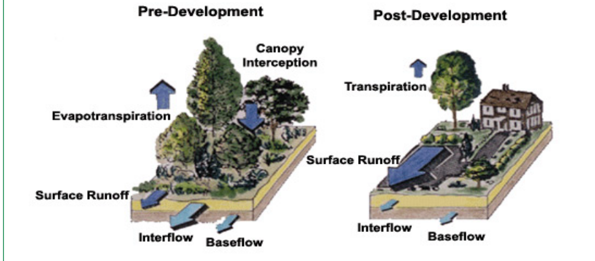
Figure 4.2.1: This diagram illustrates the increase in runoff and decrease in groundwater recharge (interflow and baseflow) that results from increased impervious surface.
